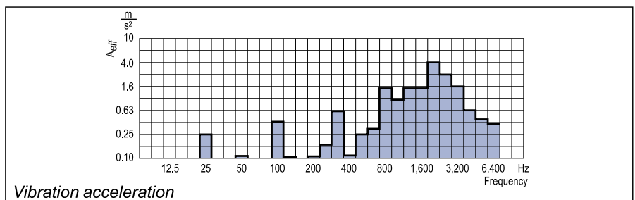
Vibration amplitude
