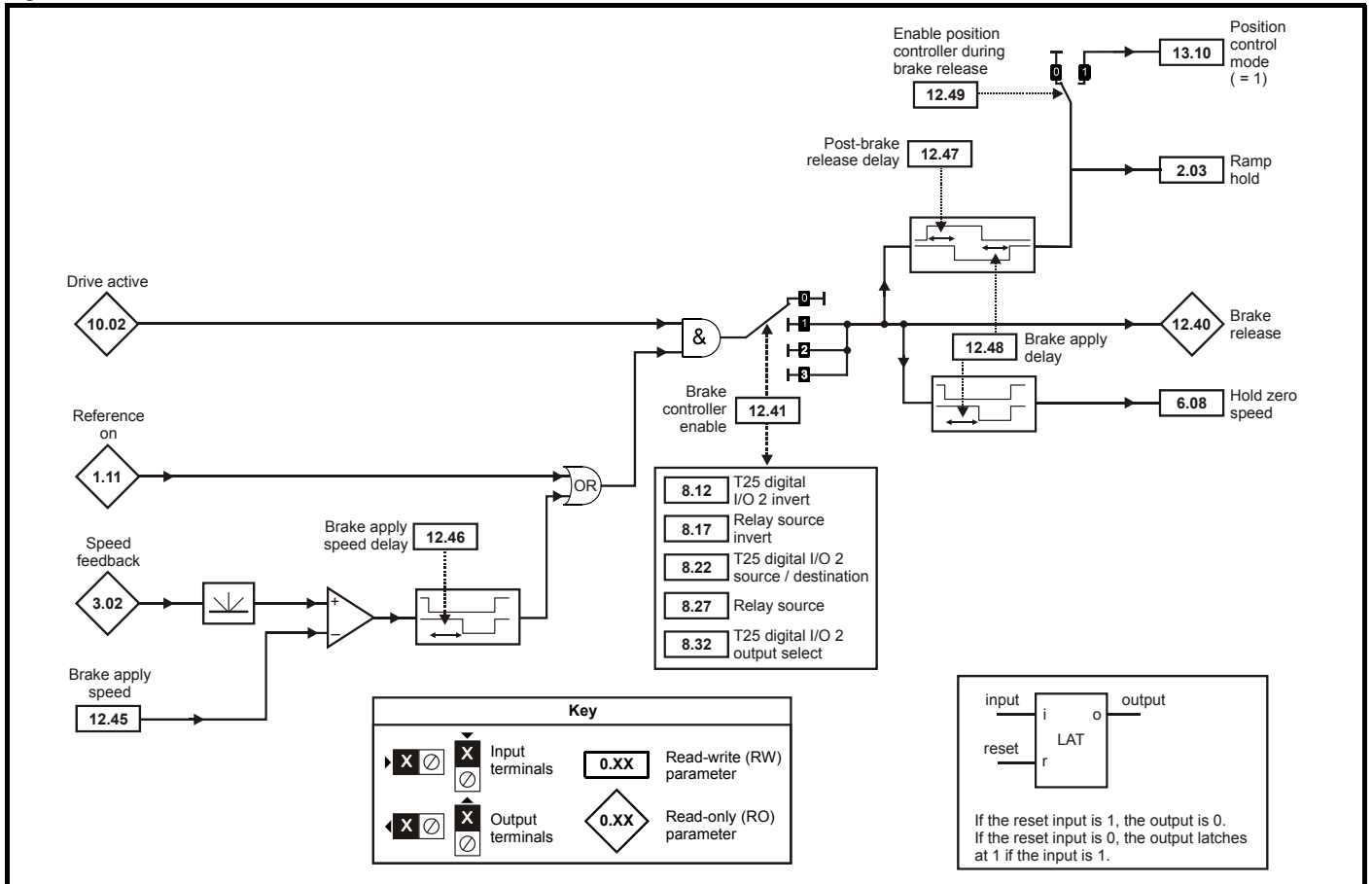
Figure 5-13 Brake function
