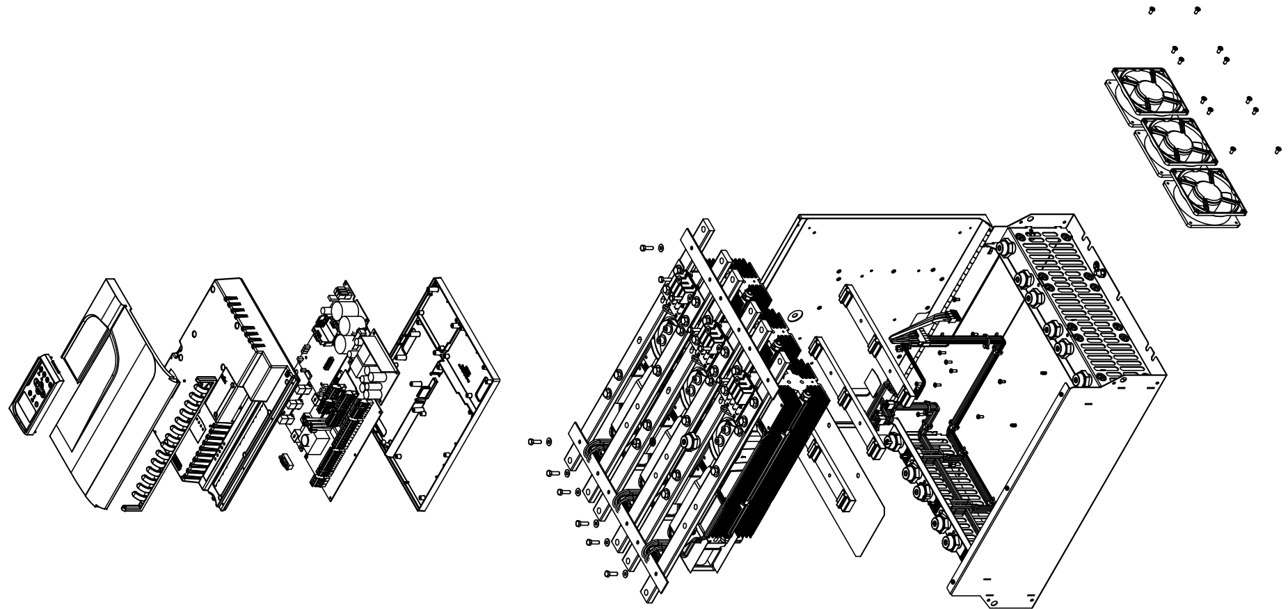
EXPLODED VIEW
