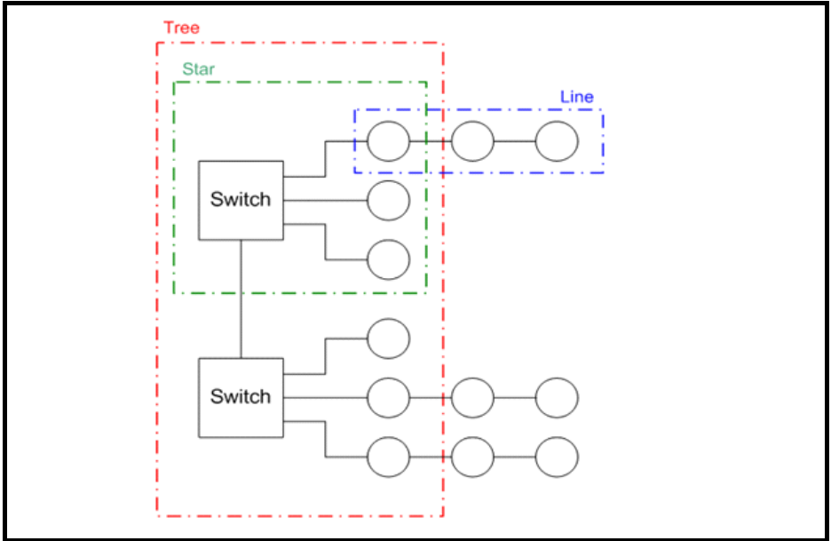
Figure 4-3 Typical network topologies
