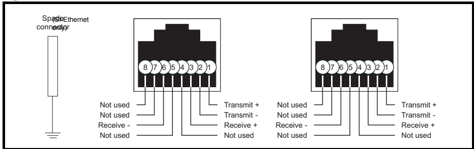
Figure 4-2 shows the electrical connections of the RJ45 connector.
