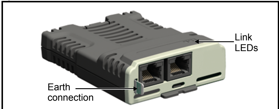
Figure 2-1 SI-Ethernet
